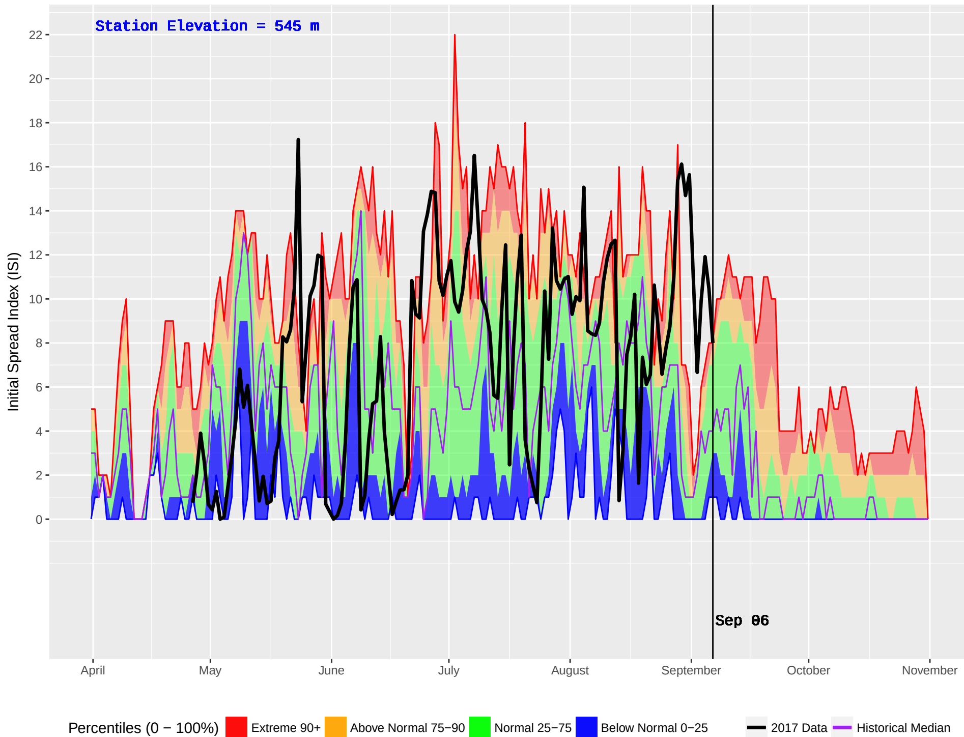
MEAGER CREEK (1083) : Historical (2010–2016) and Current (2017) Noon Initial Spread Index (ISI)
